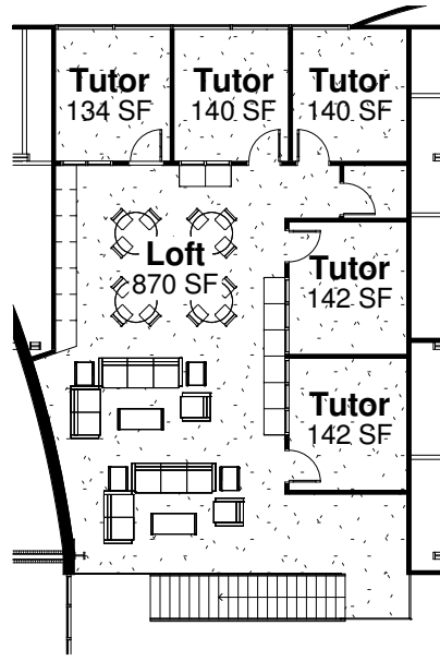
② Plan at Reading Loft 1" = 20'-0"
